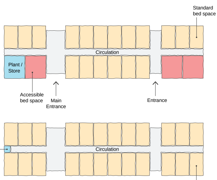
Figure A.38: Large Accommodation Block Layout (3 and 4 Storey) - Type B
